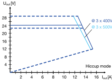
CP-T 24/10.0
