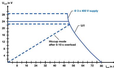
CP-T 24/40.0
