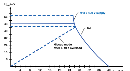
CP-T 48/20.0
